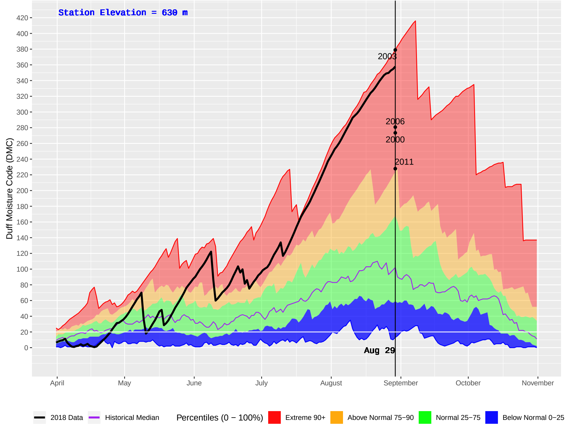
GRAND FORKS (392) : Historical (1981–2016) and Current (2018) Daily Duff Moisture Code (DMC)
